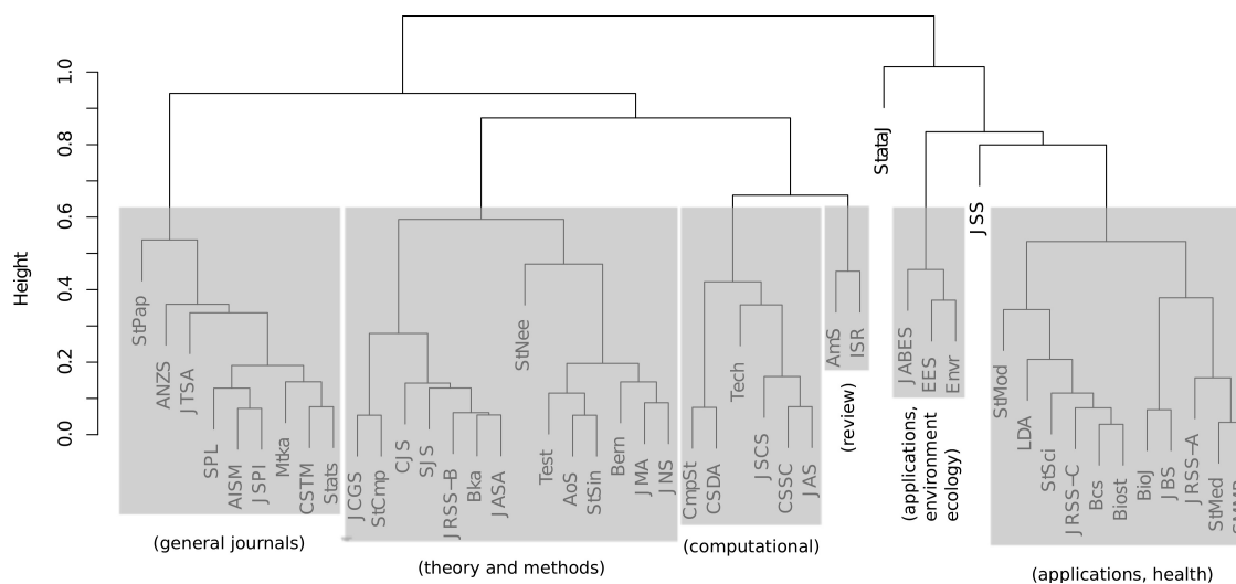
Fig. 2. Dendrogram of complete linkage hierarchical cluster analysis. Clusters obtained by cutting the dendrogram at height 0.6 are identified by grey boxes.
