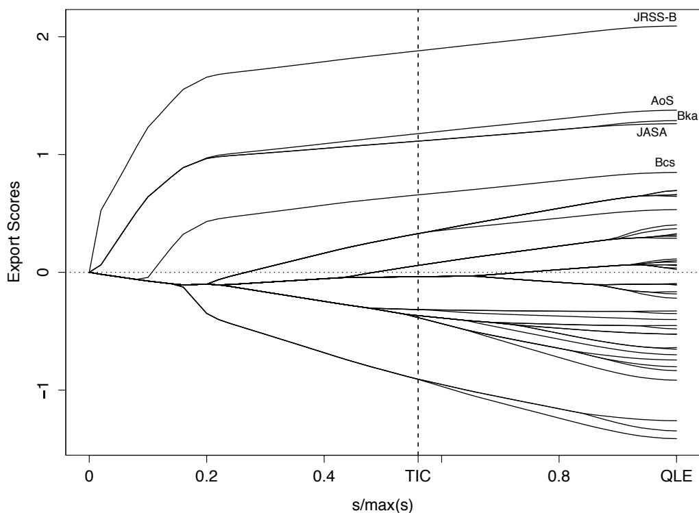
Fig. 5. Path plot of adaptive ranking lasso analysis based on Journal Citation Reports 2010 edition. QLE indicates the quasi-likelihood estimate, TIC the best ranking lasso solution according to the Takeuchi Information Criterion.
