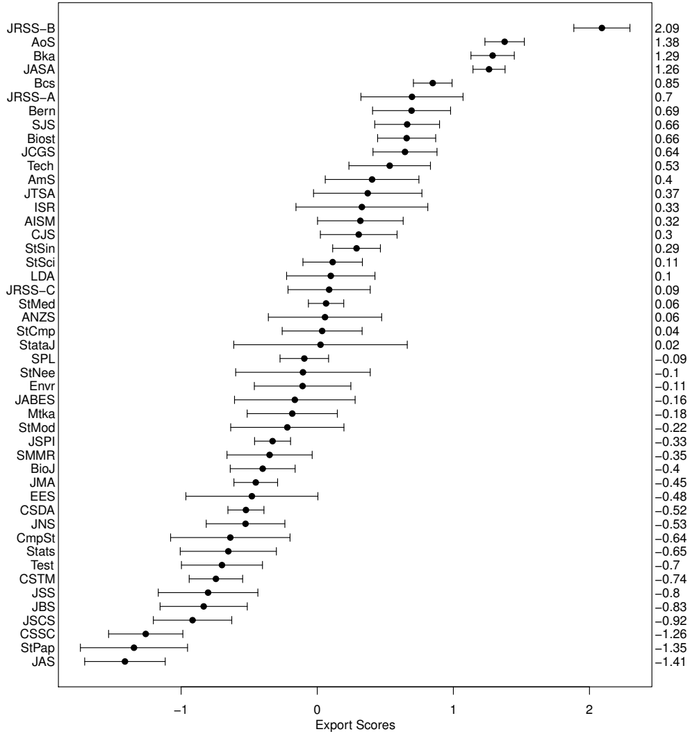
Fig. 4. Centipede plot of estimated journal export scores and 95% comparison intervals based on Journal Citation Reports 2010 edition. The error-bar limits are \hat{\mu}_i \pm 1.96 \text{qse}(\hat{\mu}_i) , with the estimated export scores \hat{\mu}_i marked by solid circles.
