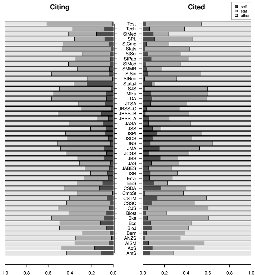
Fig. 1. Bar plots of citations made (Citing, left panel) and received (Cited, right panel) for the selected Statistics journals, as listed in Table 2, based on Journal Citation Reports 2010. For each journal, the bar displays the proportion of self-citations (dark grey), the proportion of citations made/received to/from other Statistics journals in the list (mid grey), and to/from journals not in the list (light grey).
