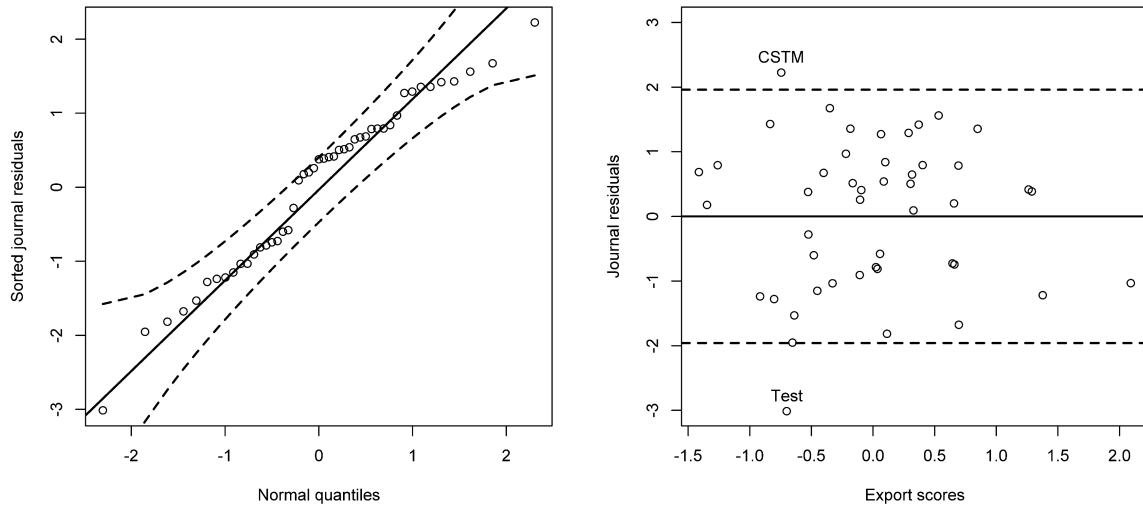
Fig. 3. Normal probability plot of journal residuals with 95% simulation envelope (left panel) and scatterplot of journal residuals versus estimated journal export scores (right panel).
