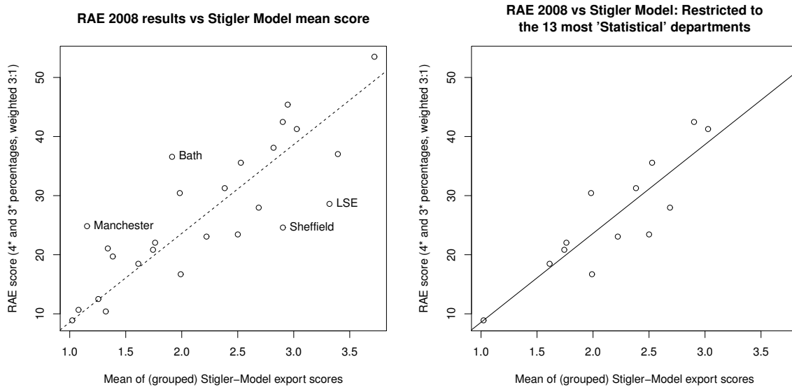
Fig. 6. Scatterplot (left panel) of RAE 2008 outcome (scores derived from the published RAE ‘Outputs’ sub-profiles) against averaged Stigler Model journal export scores for RAE-submitted papers. The 26 plotted points are the main ‘Statistics and Operational Research’ groups at UK universities; four outliers from a straight-line fit are highlighted. The right panel shows a subset of the same scatterplot, just the 13 research groups for which papers published in the 47 journals of Table 1 formed the majority of their RAE-submitted research outputs; the straight line shown in both panels is the least-squares fit to these 13 points.
