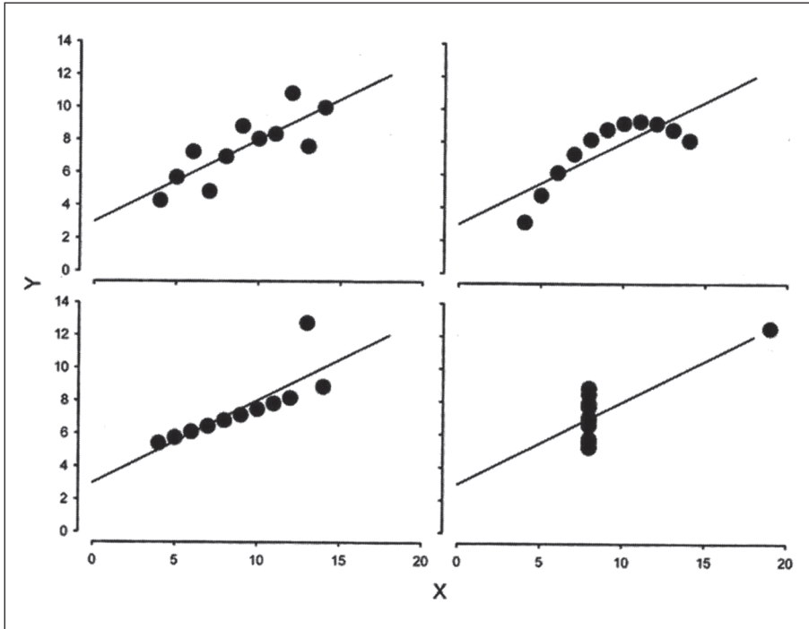
Figure 2. Anscombe's quartet. Each of the four graphs shows 11 x - y pairs and the best fitting straight line through the points. All standard statistical indicators, e.g., slope, intercept, distribution means and variances, etc. are identical for the four. (Reproduced from Anscombe, 1973, pp. 19-20, with permission).
